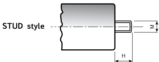
Diagram of dimensions (unit=mm) Insert and screw threads: Metric (mm), UNF (inches)
