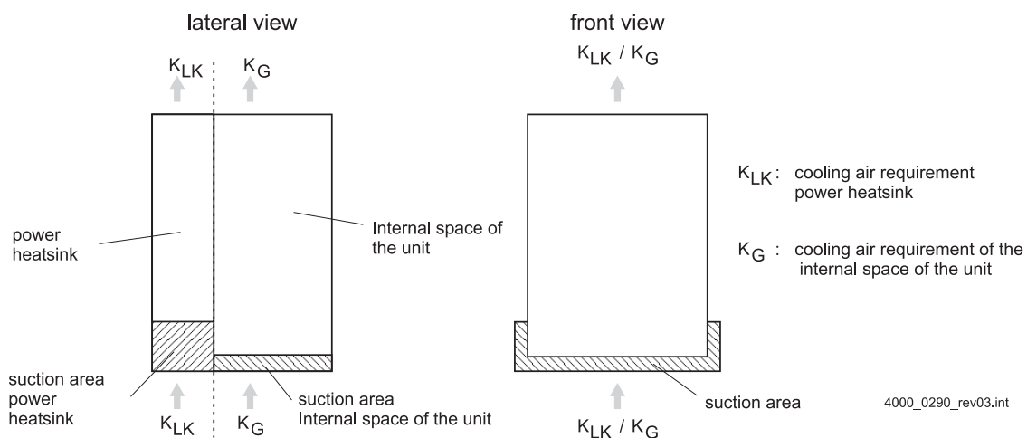
Figure 31: Cooling air requirement
