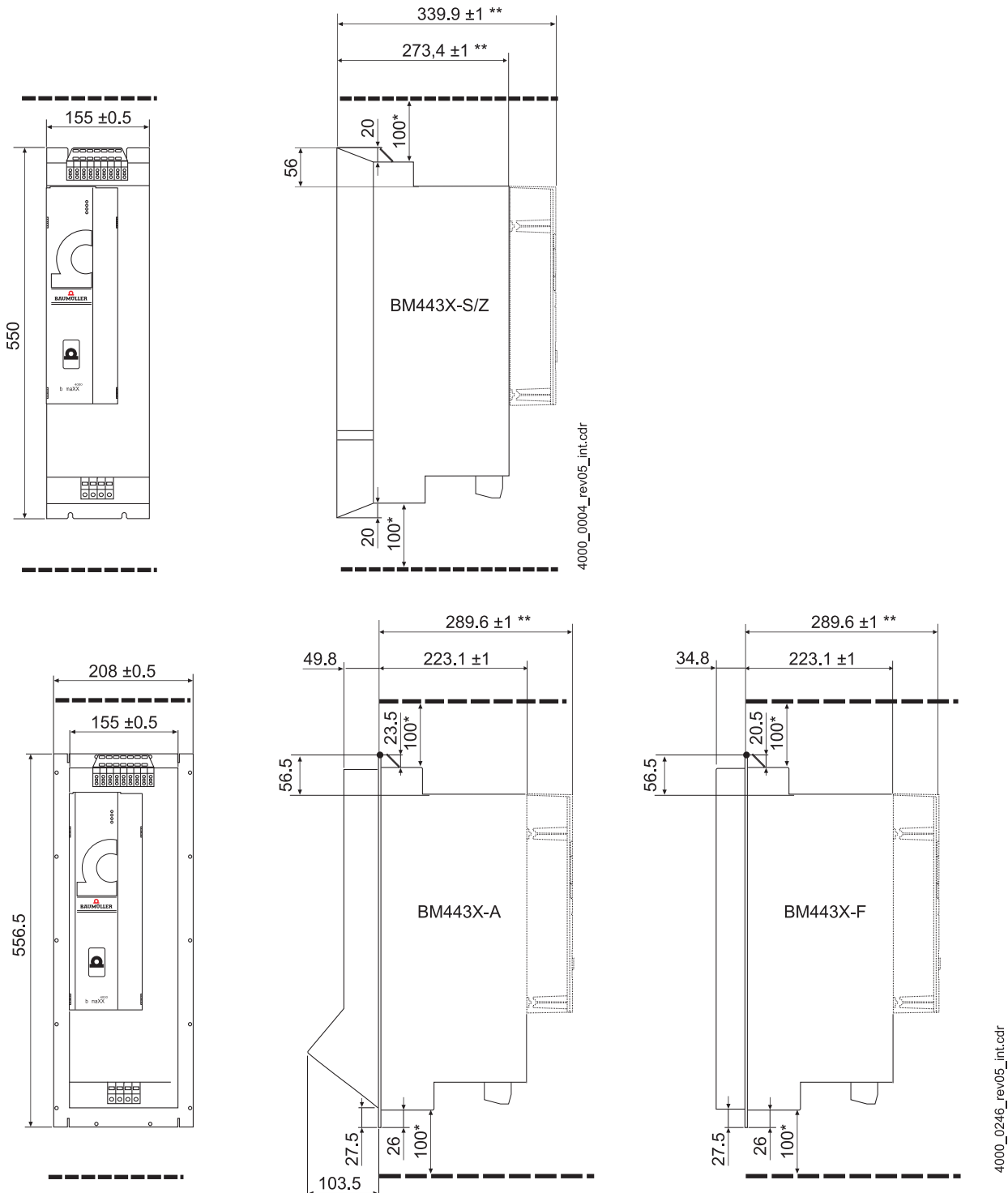
Figure 10: Dimensions BM443X-S/Z, BM443X-A/F * : Observe minimum clearance, Observe >Cooling< from page 63. **: Dimensions specified with design cover. The ES controller is not equipped with a design cover.
