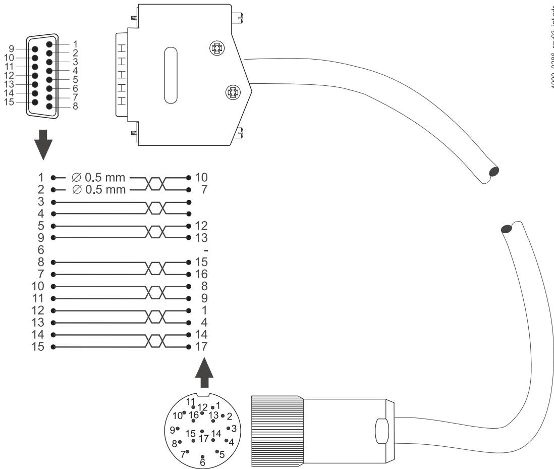
Figure 114: Cable connector for sine-cosine encoder with EnDat®-interface
