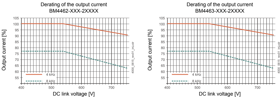
Figure 50: Derating the output current BM446X power modules
