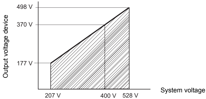
Figure 27: Reducing the output voltage in dependence with the input voltage
