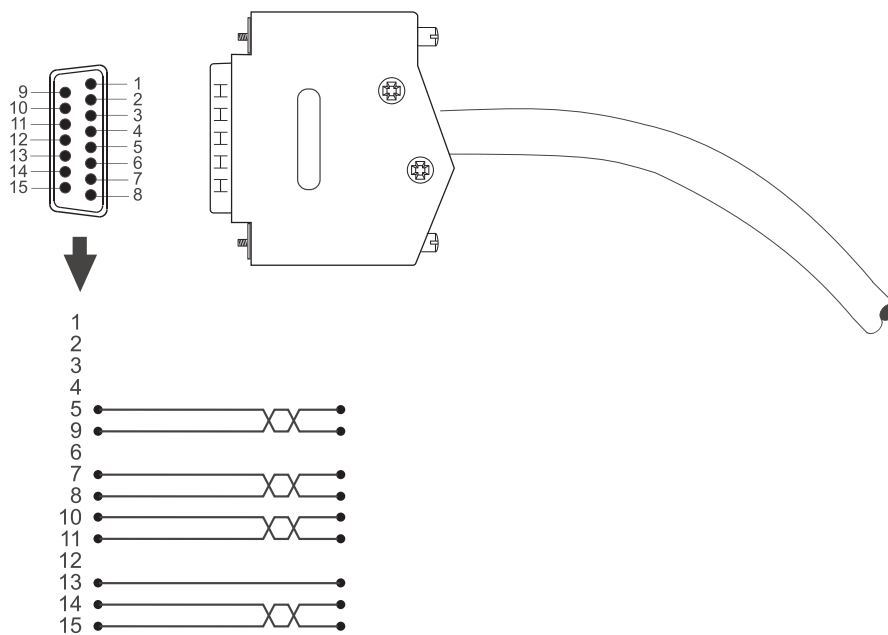
Figure 96: Connection cable BM4-F-ENC-07
