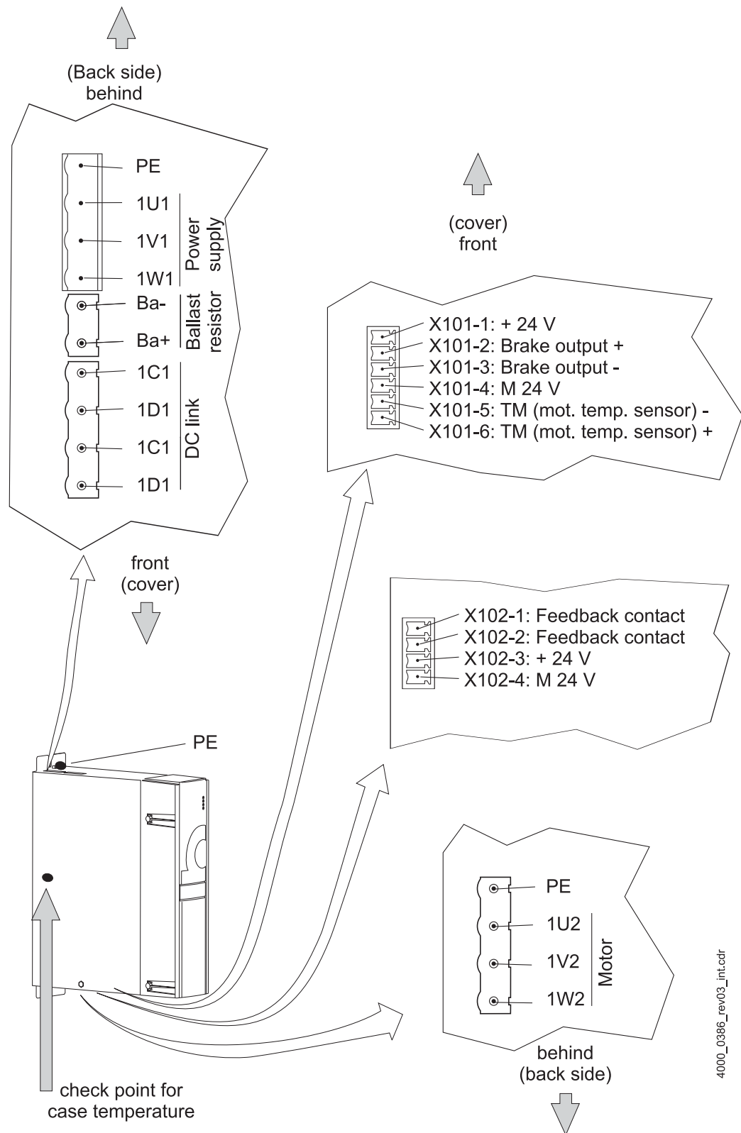
Figure 87: Electrical connections for power supply, motor, ... for BM4414
