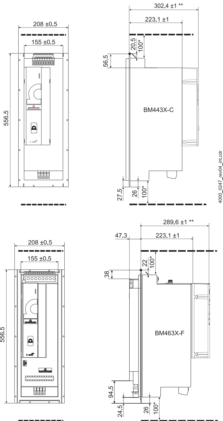
Figure 11: Dimensions BM443X-C, BM463X-F
