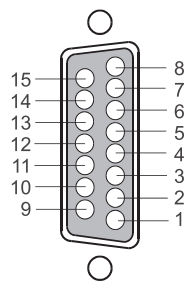
D-sub socket 15-pin
