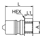
Female Thread
