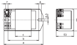
A Push-in terminals: 0.5–1.5 mm 2
